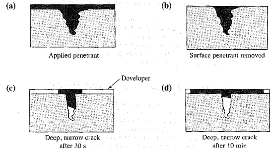
Figure 1.1: Penetration of liquid penetrant onto a surface discontinuity.
